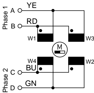
4-lead parallel / winding bipolar
