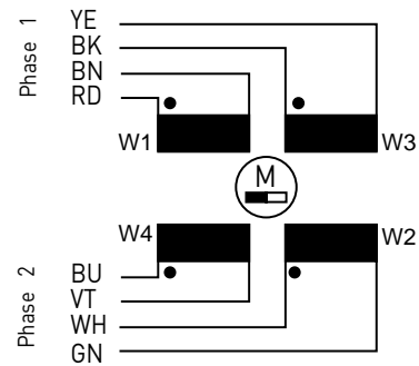
ZSS with free wire ends
