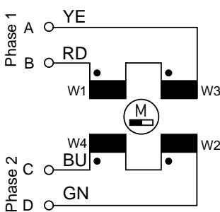
4-lead / serial windings / bipolar
